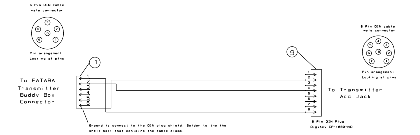
Buddy Box Interface Cable This cable is designed to connect a FUTABA FM transmitter to a MicroStar. The FUTABA transmitter will act as the slave, or student transmitter.
