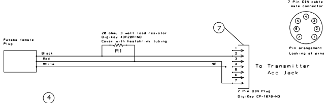
Receiver battery test cable
