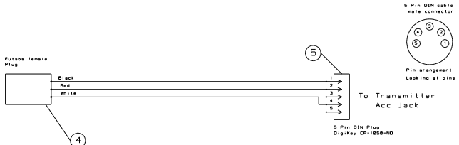
Servo Direct Drive Adapter
