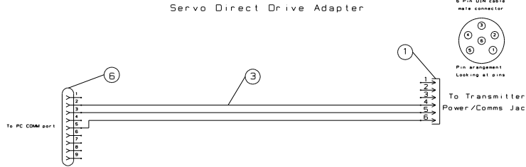
Transmitter to PC Comm Cable
