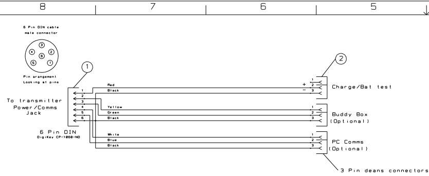
Power/Comms interface cable
