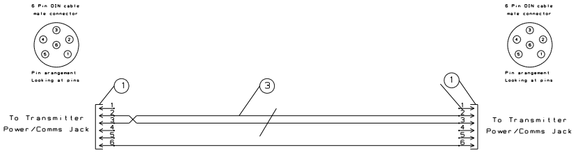
Buddy Box Interface Cable This cable is designed to connect MicroStar to MicroStar only!
